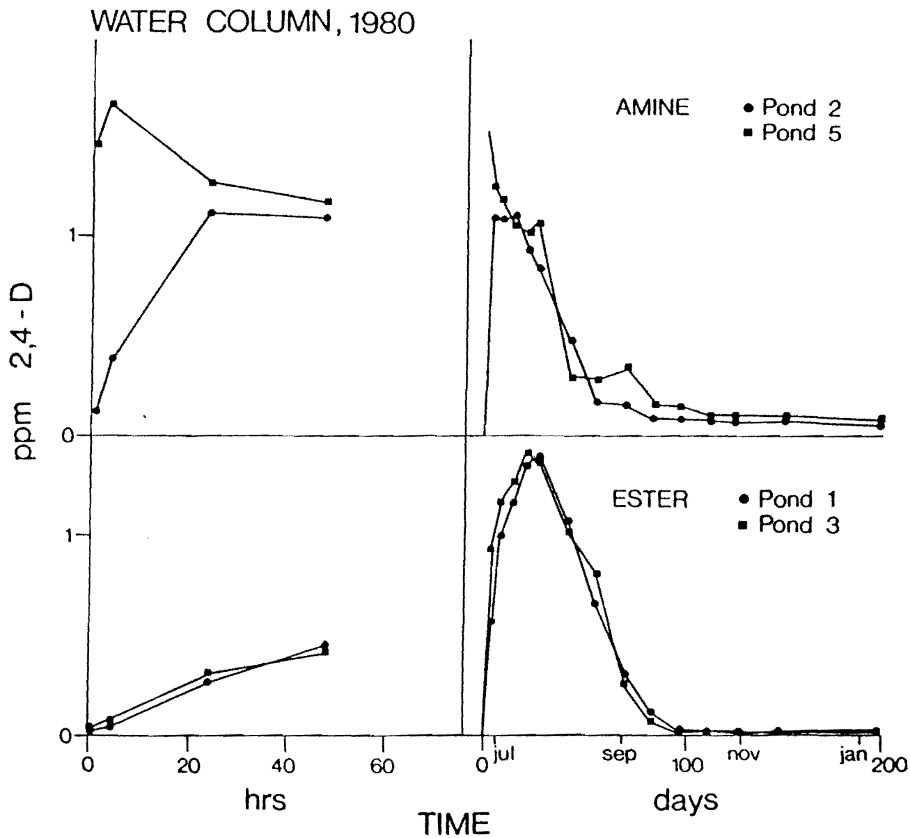
FIGURE 1. 2,4-D concentrations in the water (1980).
